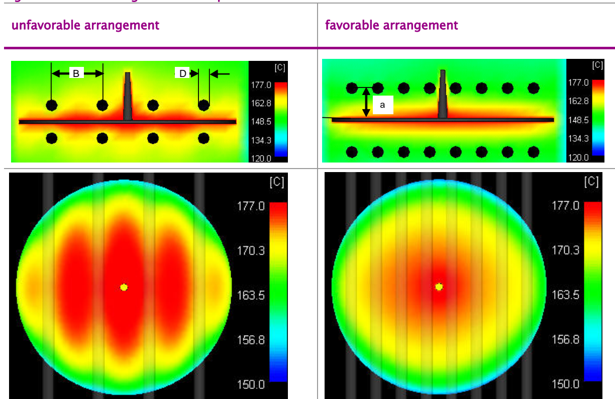
Fig. 8: Different arrangement of temperature control channels to the surface of the molded item
