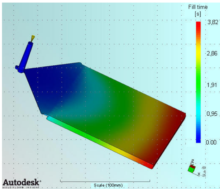
Fig. 9: Plaque 130 x 130mm 2
