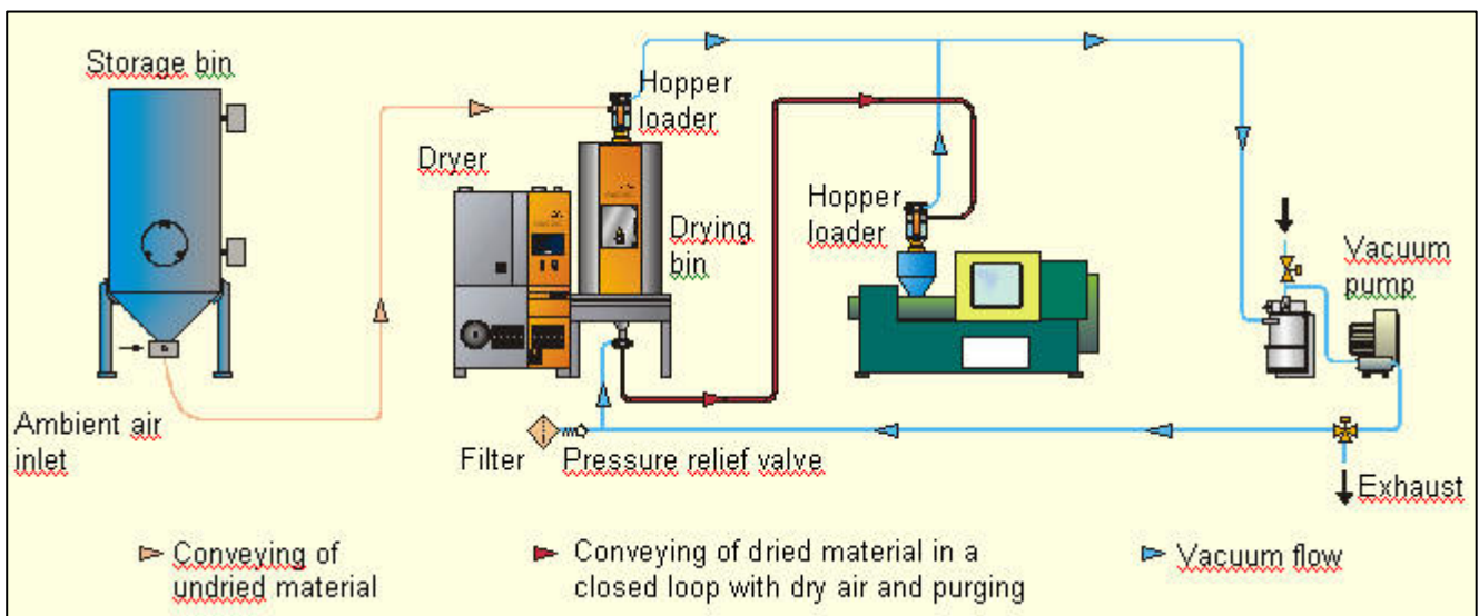
Fig.1: Drying diagram for PPA (Motan)
