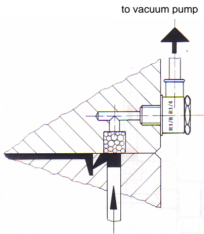
Fig. 7: Venting diagram (Bawema)
