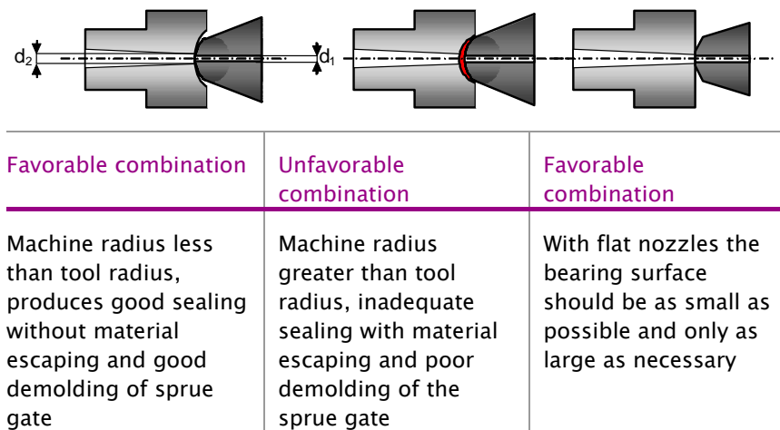
Fig. 3: Coordinating the radii of machine nozzle and sprue bushing
