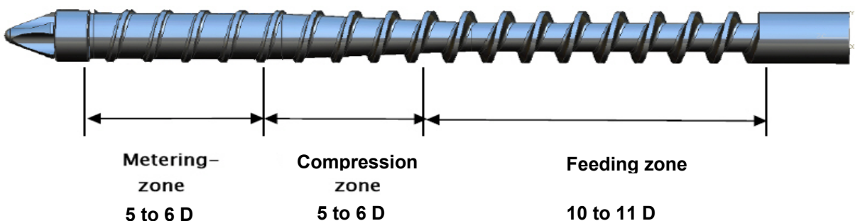
Fig. 2: Universal 3-zone screw
