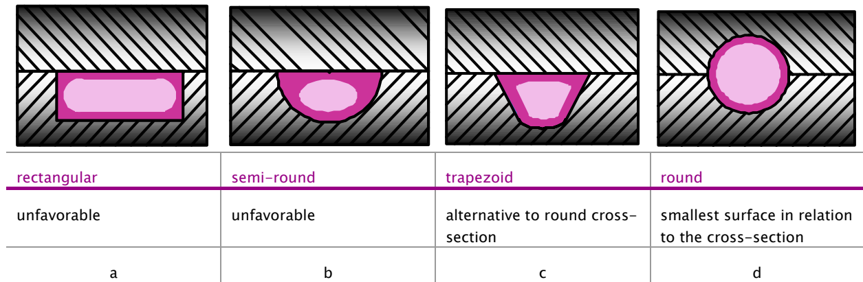
Fig. 4: Different cross-sections of sprue manifolds
